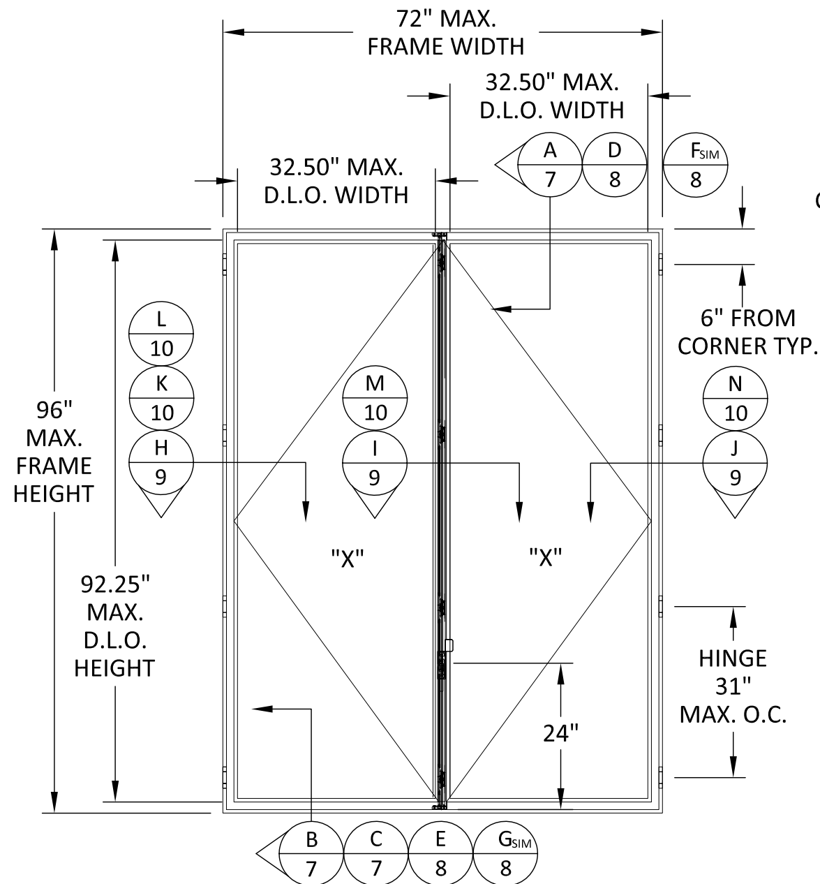
ELEVATION OUTSWING CASEMENT TWIN WINDOW INSIDE OR OUTSIDE GLAZED
