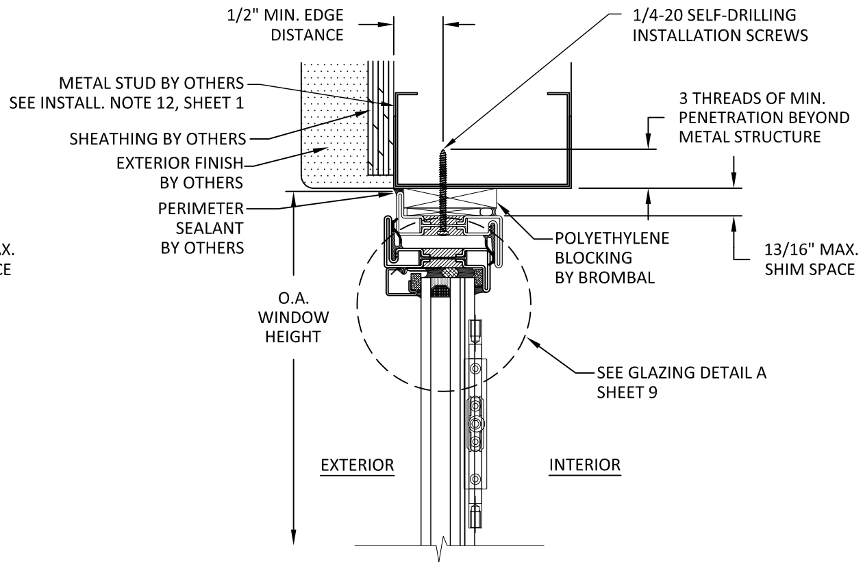
F 8 VERTICAL SECTION SINGLE HEAD - METAL STUD FRAME OUTSIDE GLAZED
