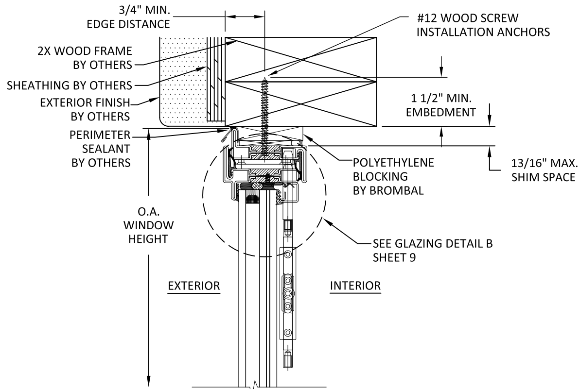
A 7 VERTICAL SECTION TWIN HEAD - 2X WOOD FRAME INSIDE GLAZED
