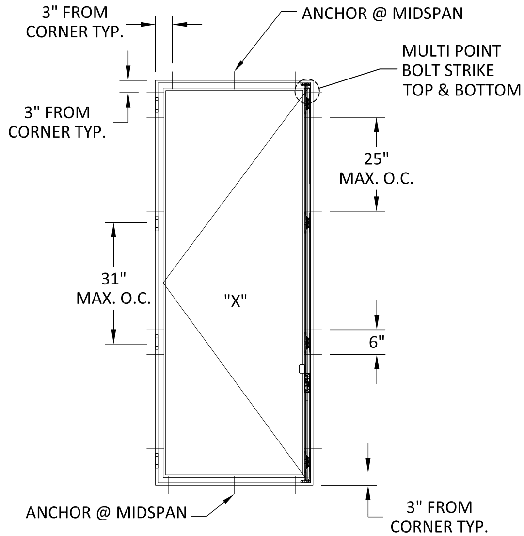
ANCHOR LAYOUT OUTSWING CASEMENT SINGLE WINDOW INSIDE OR OUTSIDE GLAZED
