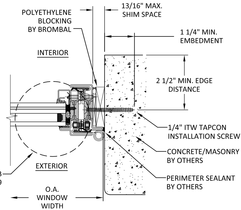
J 9 HORIZONTAL SECTION HINGE JAMB - CONCRETE/MASONRY INSIDE GLAZED
