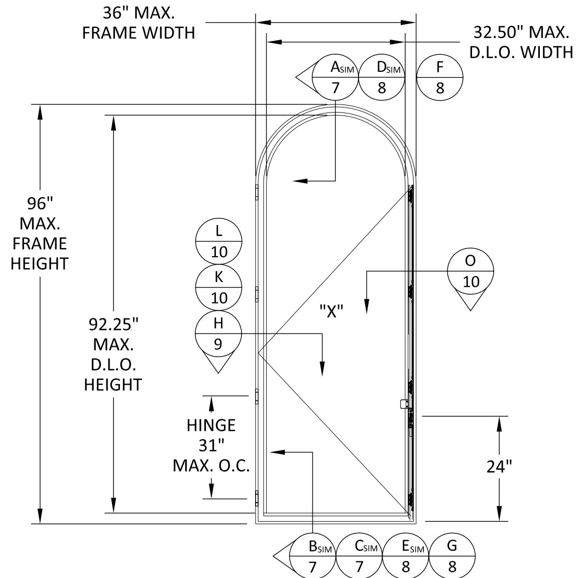
ELEVATION OUTSWING ARCHED SINGLE WINDOW INSIDE OR OUTSIDE GLAZED
