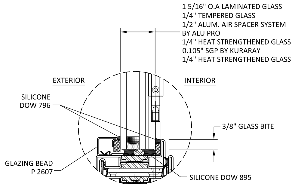
GLAZING DETAIL A OUTSIDE GLAZED
