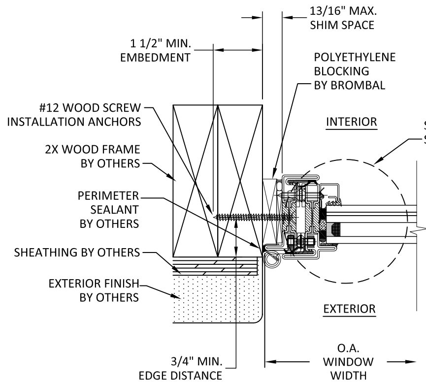
H 9 HORIZONTAL SECTION HINGE JAMB - 2X WOOD FRAME INSIDE GLAZED
