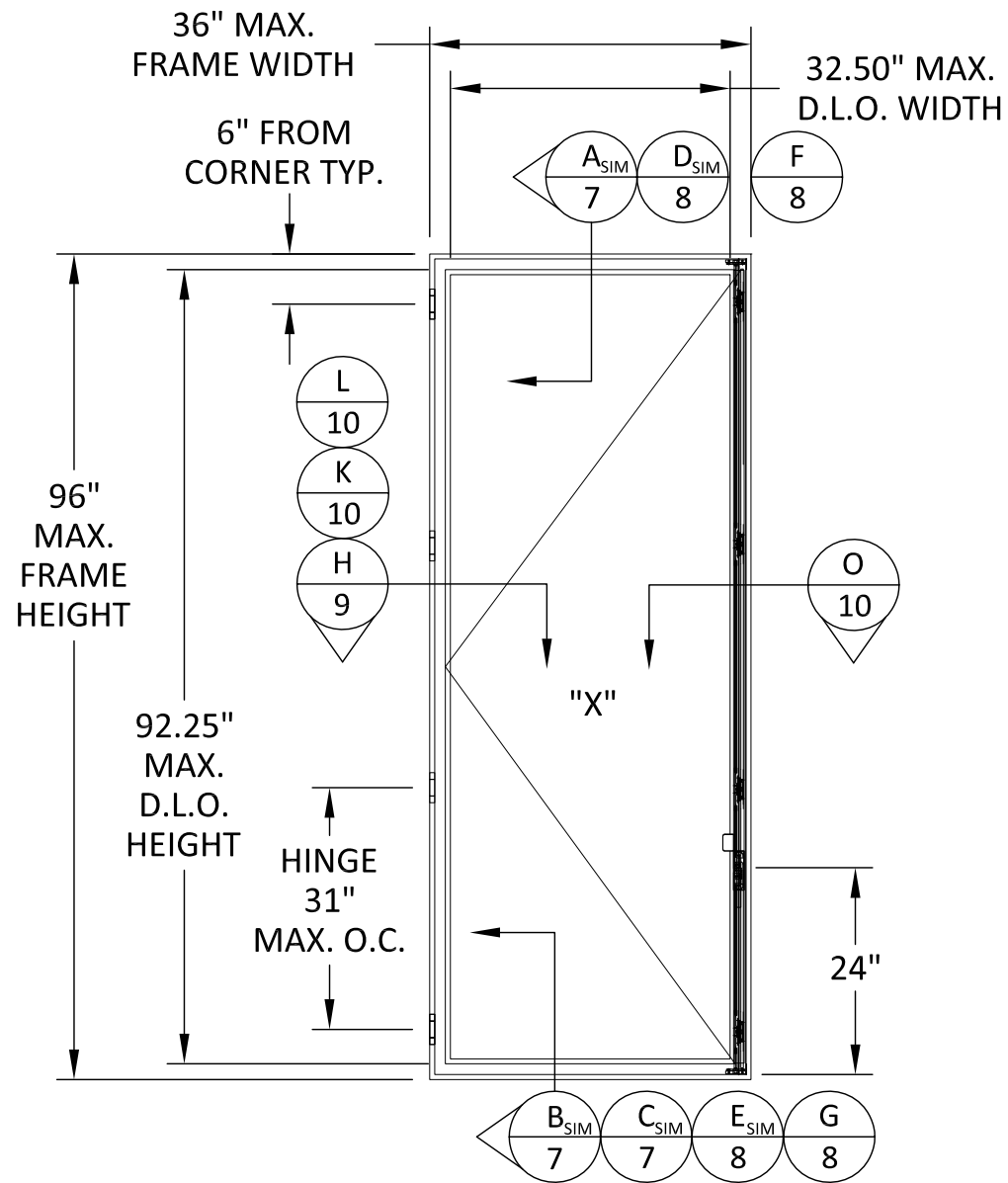
ELEVATION OUTSWING CASEMENT SINGLE WINDOW INSIDE OR OUTSIDE GLAZED
