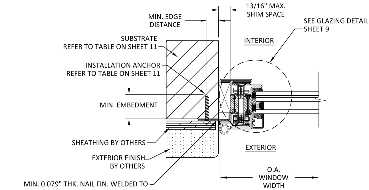
P 11 HORIZONTAL SECTION NAIL FIN INSTALLATION TYP. INSTALLATION - HEAD/JAMB/SILL
