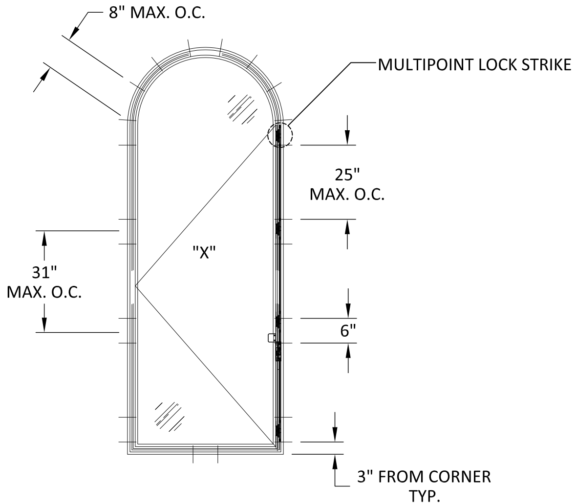
ANCHOR LAYOUT OUTSWING ARCHED SINGLE WINDOW INSIDE OR OUTSIDE GLAZED
