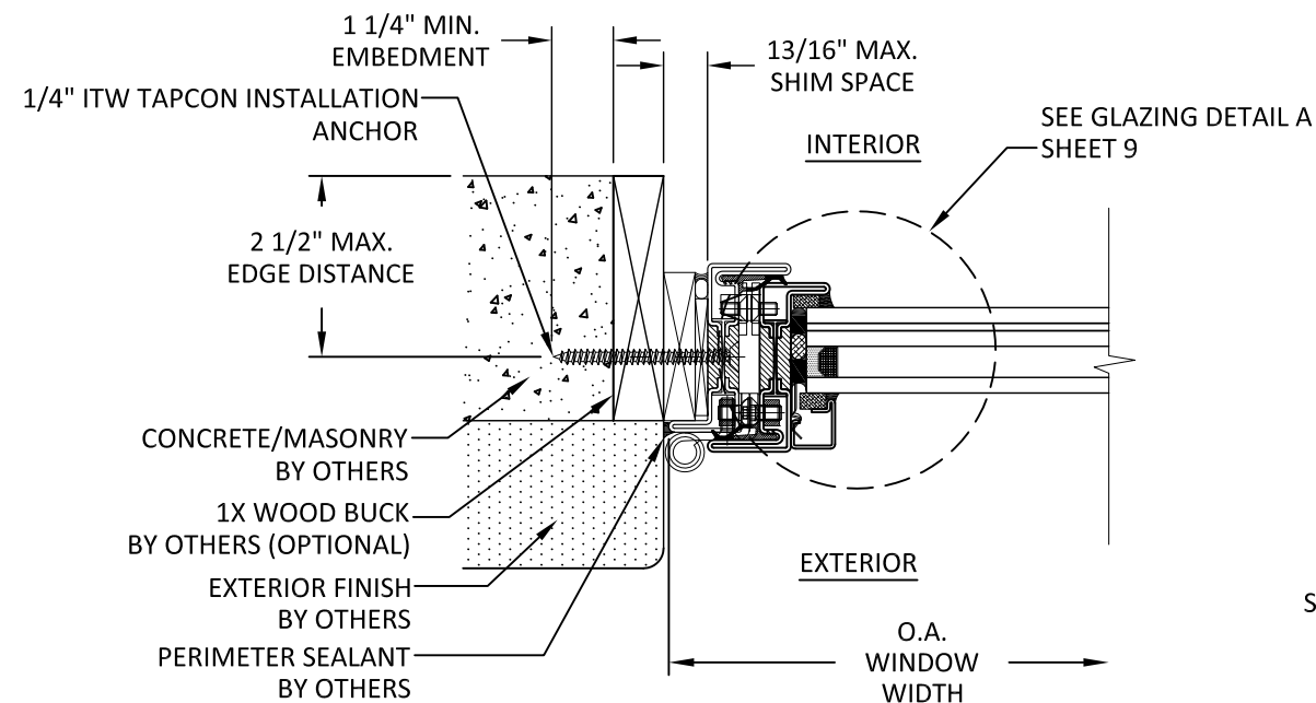
L 10 HORIZONTAL SECTION HINGE JAMB - 1X WOOD BUCK / CONCRETE/MASONRY OUTSIDE GLAZED
