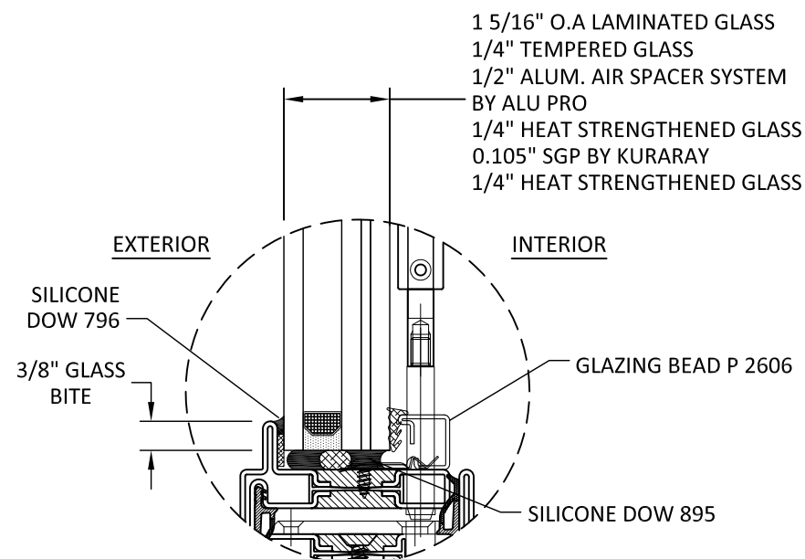
GLAZING DETAIL B INSIDE GLAZED
