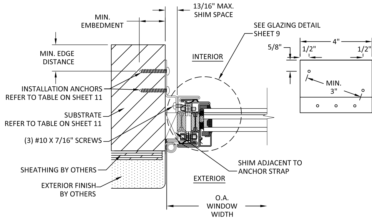
R 11 HORIZONTAL SECTION THRU STRAP INSTALLATION TYP. INSTALLATION - HEAD/JAMB/SILL
